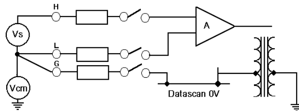
FIGURE 6.8 3-POLE COMMON MODE SIGNAL REJECTION CIRCUIT
