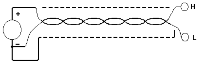
FIGURE 6.2 2 POLE THERMOCOUPLE CONNECTIONS
