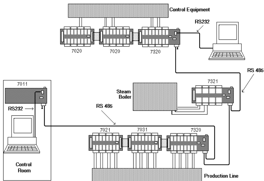
FIGURE 1.1 TYPICAL DATASCAN INSTALLATION
